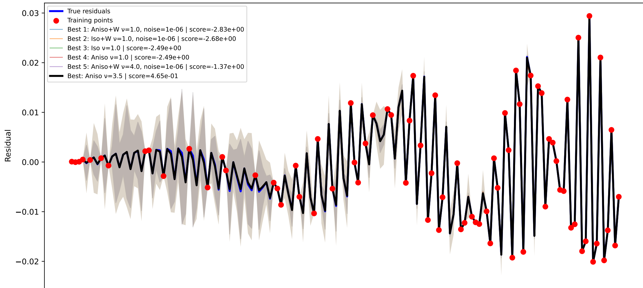
GPR kernel comparison node=37 RMSE=1.486e-04, train RMSE=1.146e-11
